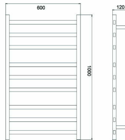
Round Heated Towel Rail 9 Bars(Exposed/Concealed Power Cord)
