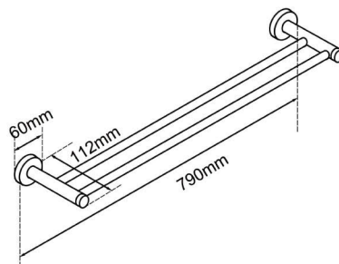
Double Towel Rail 790mm (Cuttable)
