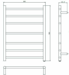
Round Heated Towel Rail 7 Bars(Exposed/Concealed Power Cord)
